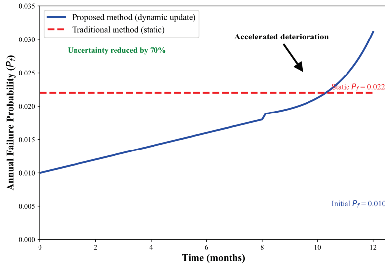
Figure 2 Trend chart of annual failure probability P_f changing with time
